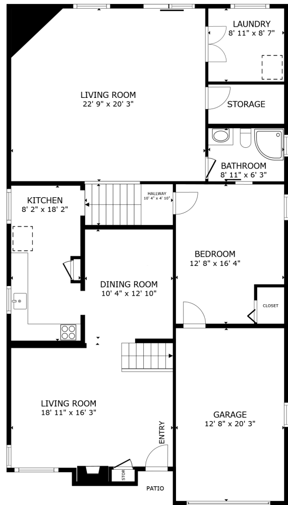
FLOOR 1
