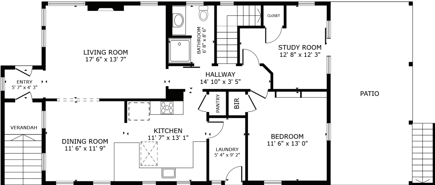
FLOOR 1
