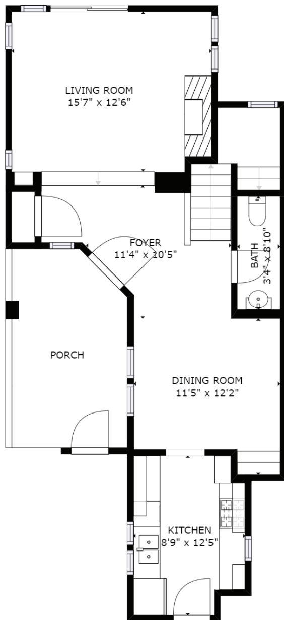
FLOOR 1
